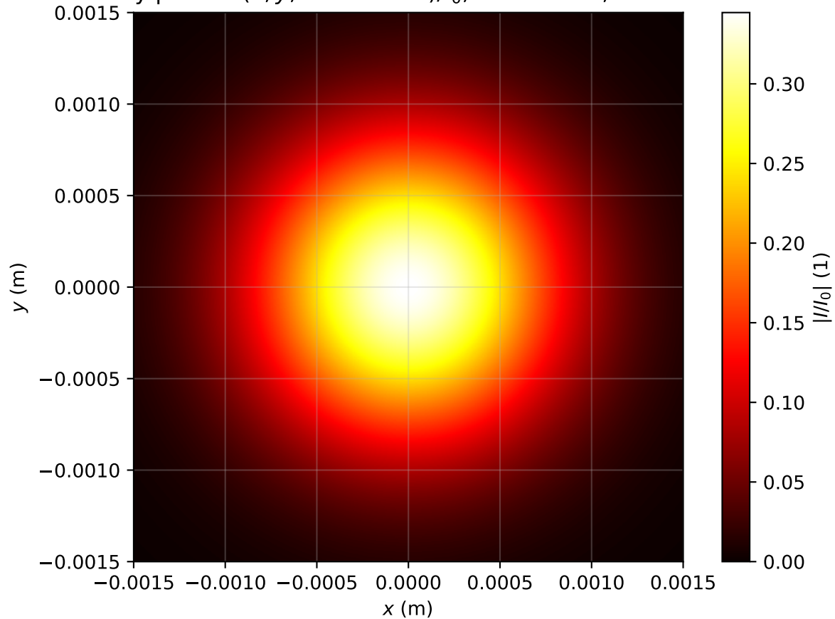
Intensity profile I(x, y, z = 2.946m)/I_0 , P_{in}=0.1P_{cr} , artificial time
